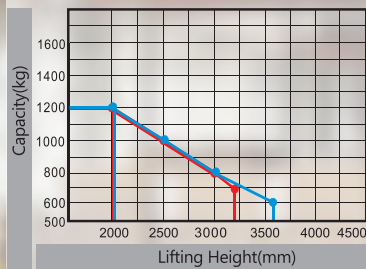
Load Curve
